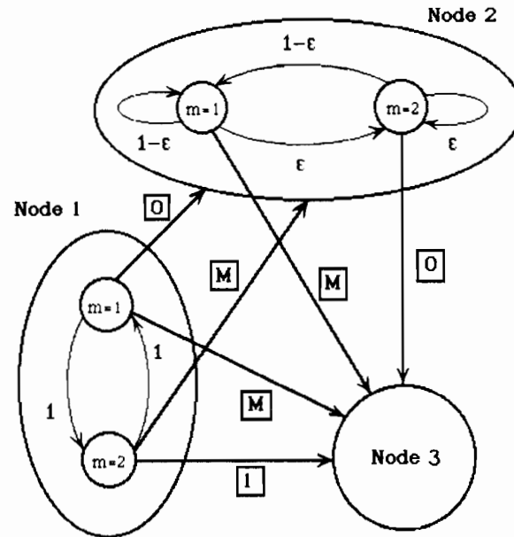
Figure 4. Example of a 3-node network in which a state color (here, that of the 1st state at node 1) can change from green to red and back to green. This is a combined graph in which states at nodes 1 and 2 are shown as small circles. Nodes 1 and 2 are shown as large ellipses. Arcs are shown in bold and arc costs are shown inside boxes. Also shown are the dynamics of the Markov processes at nodes 1 and 2 and the transition probabilities.
