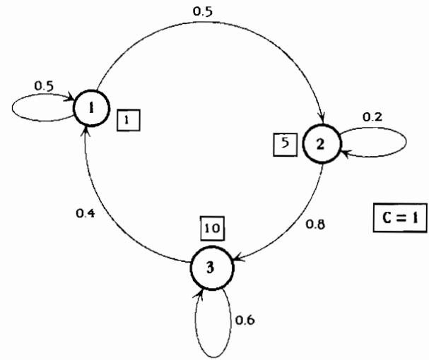
Figure 2. Example for the comparison of procedures SA and PI.
