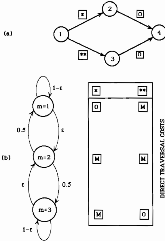
Figure 3. An example in which the naive procedure performs arbitrarily poorly.
